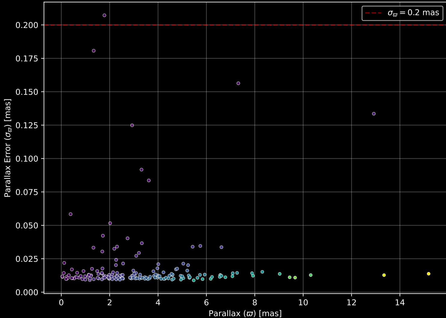
APOGEE DR17 Field: [085+59_MGA] Parallax Quality (n= 180)
