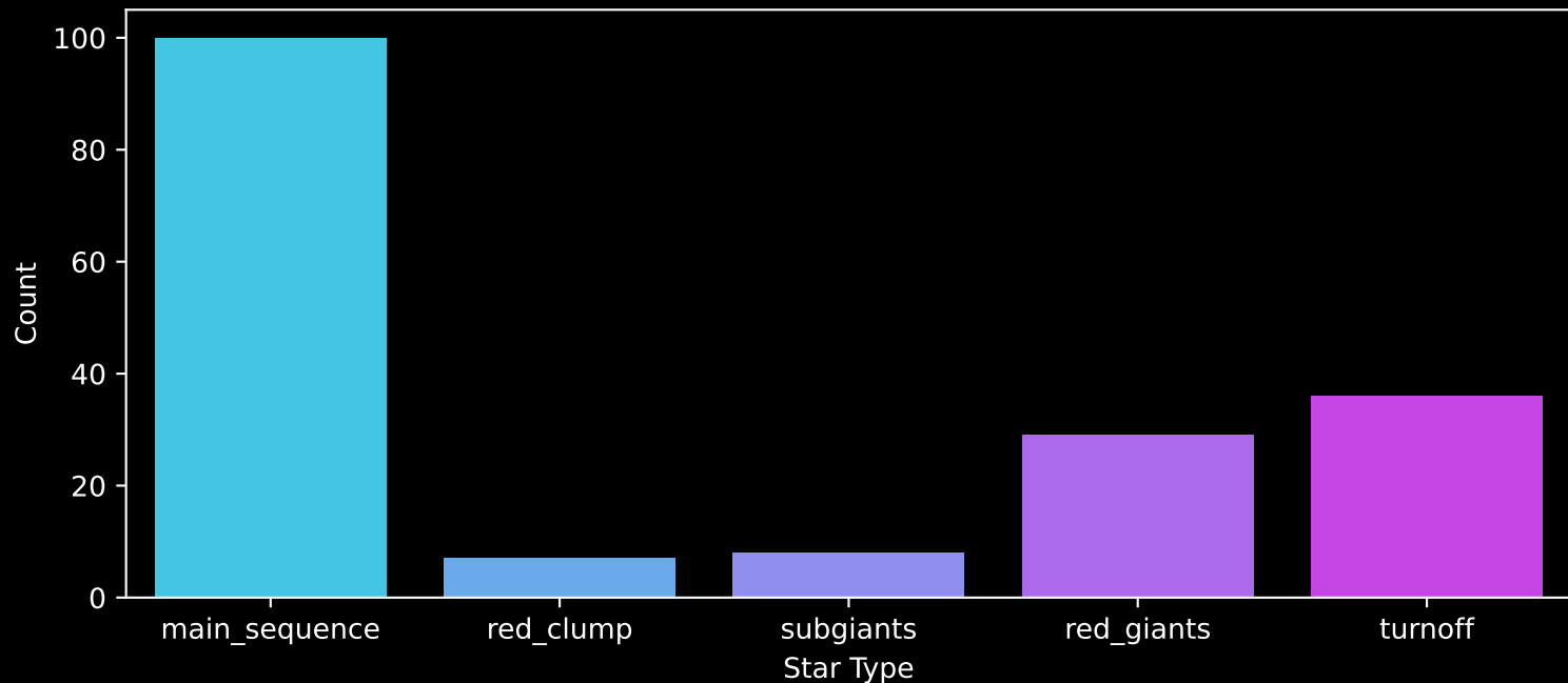
APOGEE DR17 Field: [085+59_MGA] Count plot of Star Type
