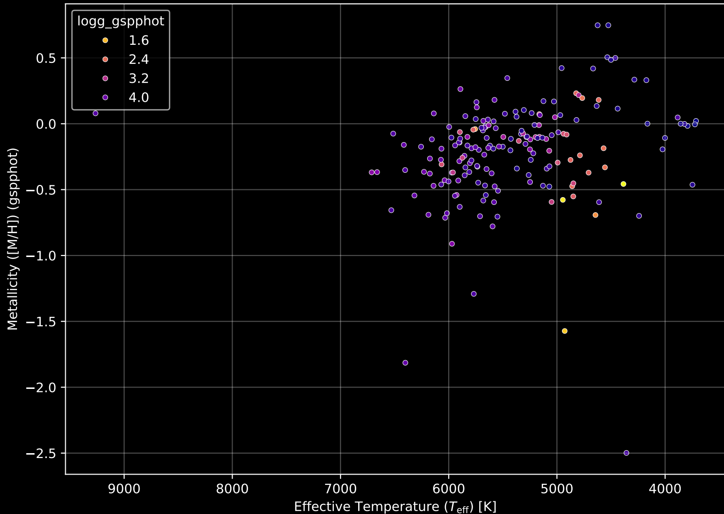
APOGEE DR17 Field: [085+59_MGA] Stellar Population Parameters (n= 180)
