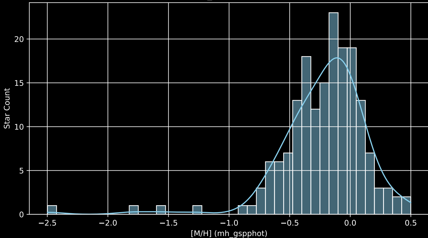
APOGEE DR17 Field: [085+59_MGA [M/H] (mh_gspphot) (n= 177)
