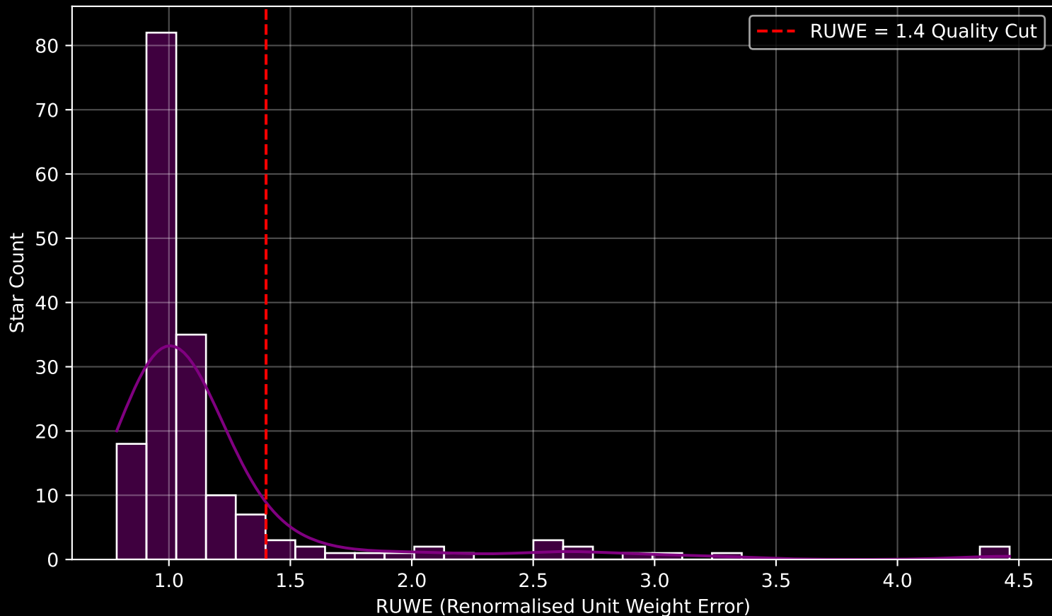
GAPOGEE DR17 Field [085+59_MGA] RUWE Distribution (n= 173)
