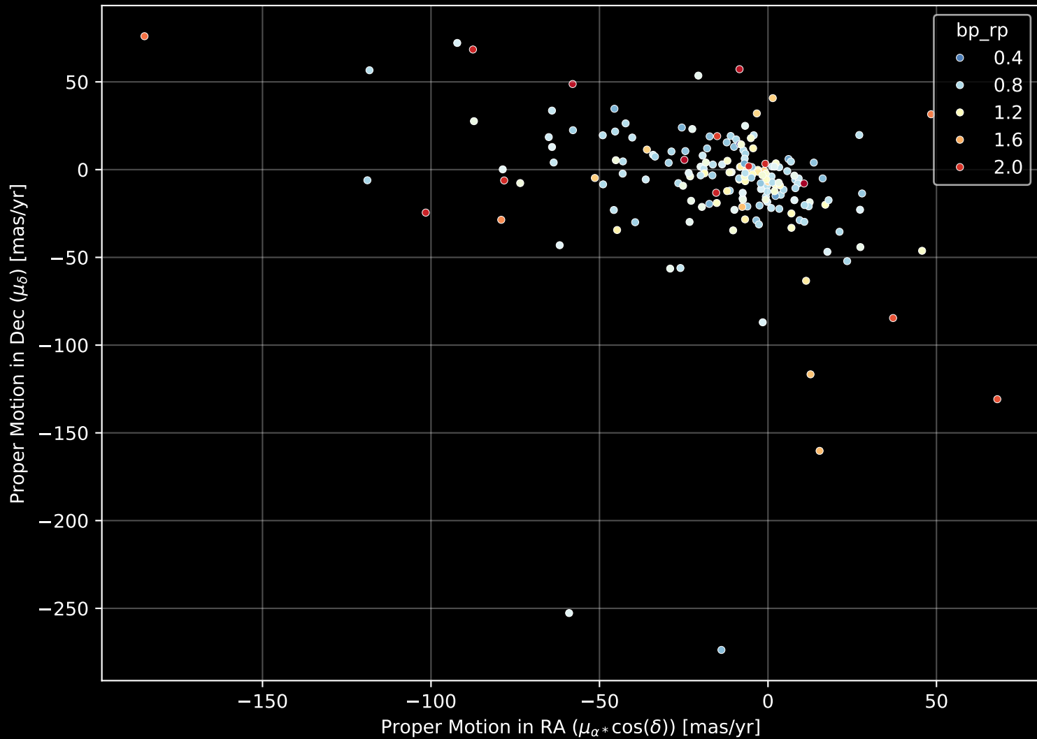
APOGEE DR17 Field: [085+59_MGA] Proper Motion Diagram (n= 180)
