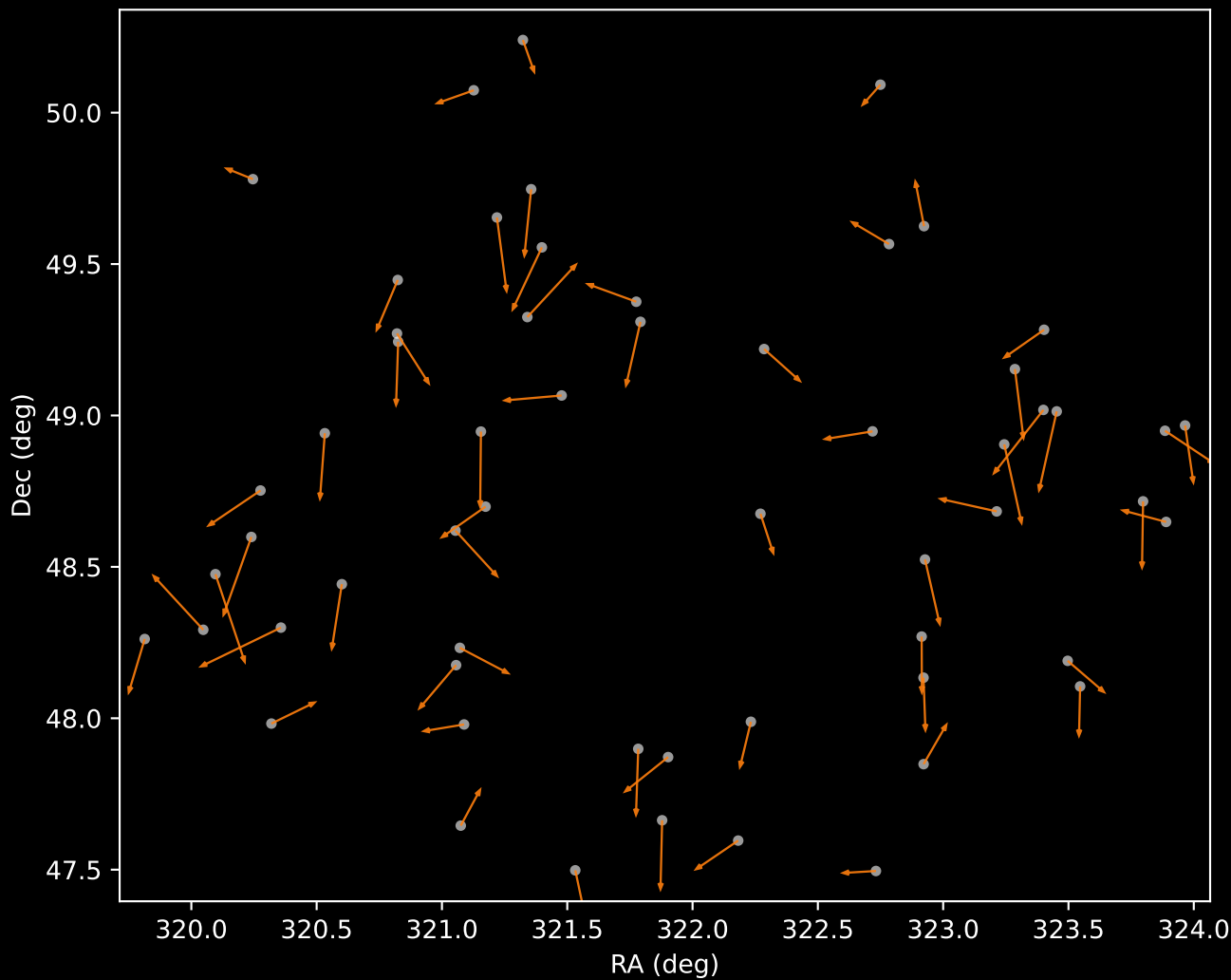
APOGEE DR17 Cluster 2 Proper Motion Vectors (n=58)
